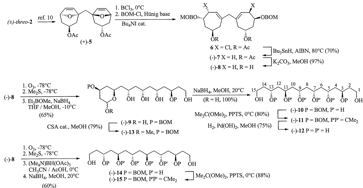
Scheme 2. New strategy for the expeditious preparation of long-chain polyketides; AIBN: \text{Me}_2\text{C}(\text{CN})\text{N}=\text{NC}(\text{CN})\text{Me}_2 , BOM = \text{PhCH}_2\text{OCH}_2 , CSA: camphorsulfonic acid, Hünig base: (i\text{Pr})_2\text{NEt} , PPTS: pyridinium p -toluenesulfonate
